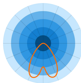
Double asymmetric 20°
