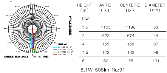
10° LED 4000K CODE:AA8888888
