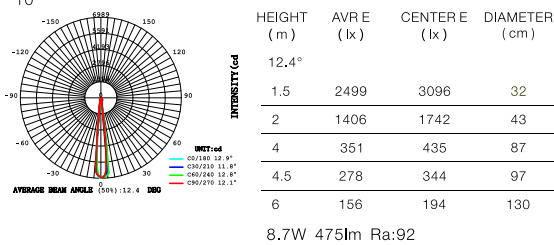
10° LED 3000K CODE:AA8888888
