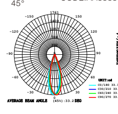
LED 4000K CODE:AA8888888
