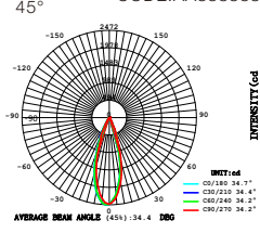
LED 3000K CODE:AA8888888
