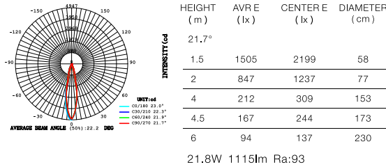
15° LED 3000K CODE:AA8888888
