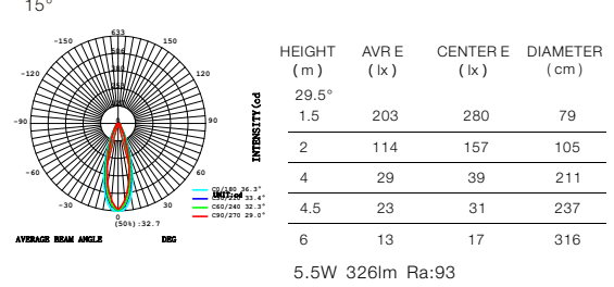
LED 4000K CODE:AA8888888
