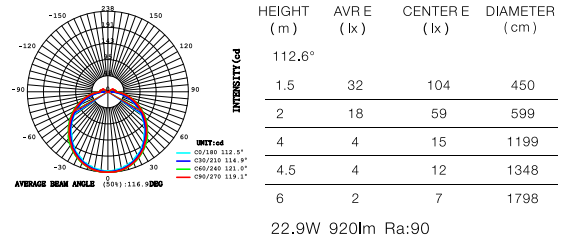
120° ● LED 4000K CODE:AA8888888
