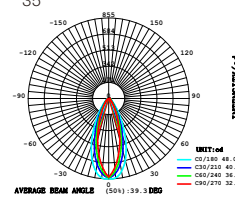
LED 4000K CODE:AA8888888
